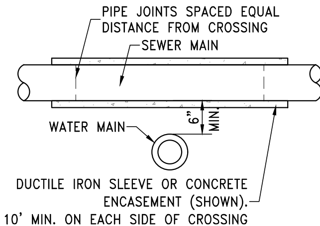
SEWER MAIN CROSSING WATER MAIN (ALT.)
